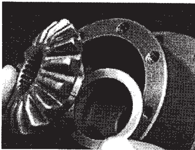
Figure 8 Place washer and former top gear into case
